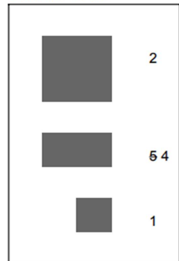
Asteroid Count
